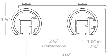
DOUBLE SUPPORT
