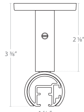
CEILING SUPPORT
