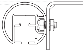
CEILING SUPPORT
