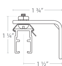
SHORT SUPPORT
