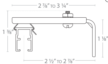
ADJUSTABLE SUPPORT
