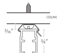
CEILING SUPPORT
