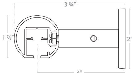
WALL SUPPORT
