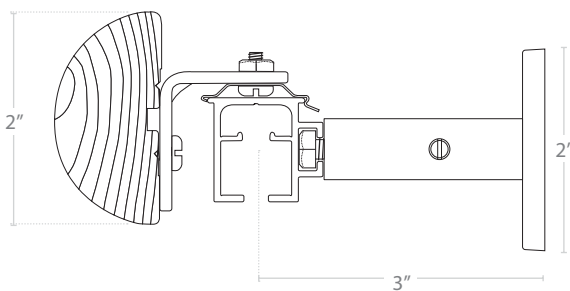
WALL SUPPORT
