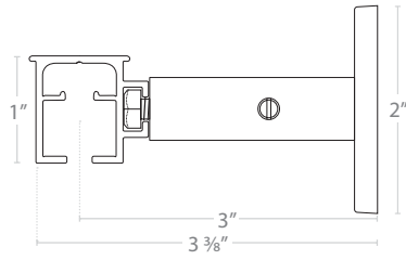
WALL SUPPORT
