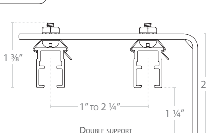
DOUBLE SUPPORT
