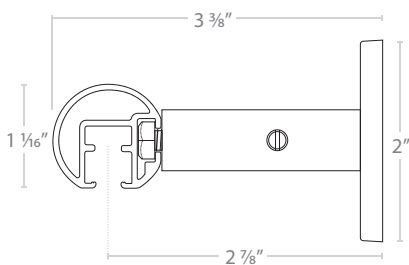
WALL SUPPORT
