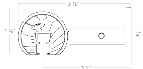
WALL SUPPORT
